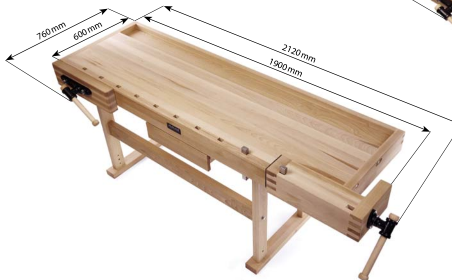
SHORT version of PREMIUM ORIGINAL workbench KURZE Version der PREMIUM ORIGINAL Werkbank
