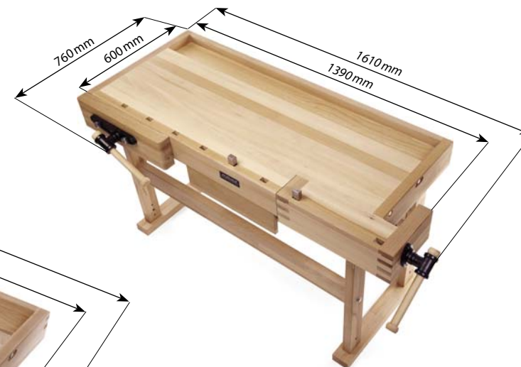
SHORT version of PREMIUM ORIGINAL workbench KURZE Version der PREMIUM ORIGINAL Werkbank
